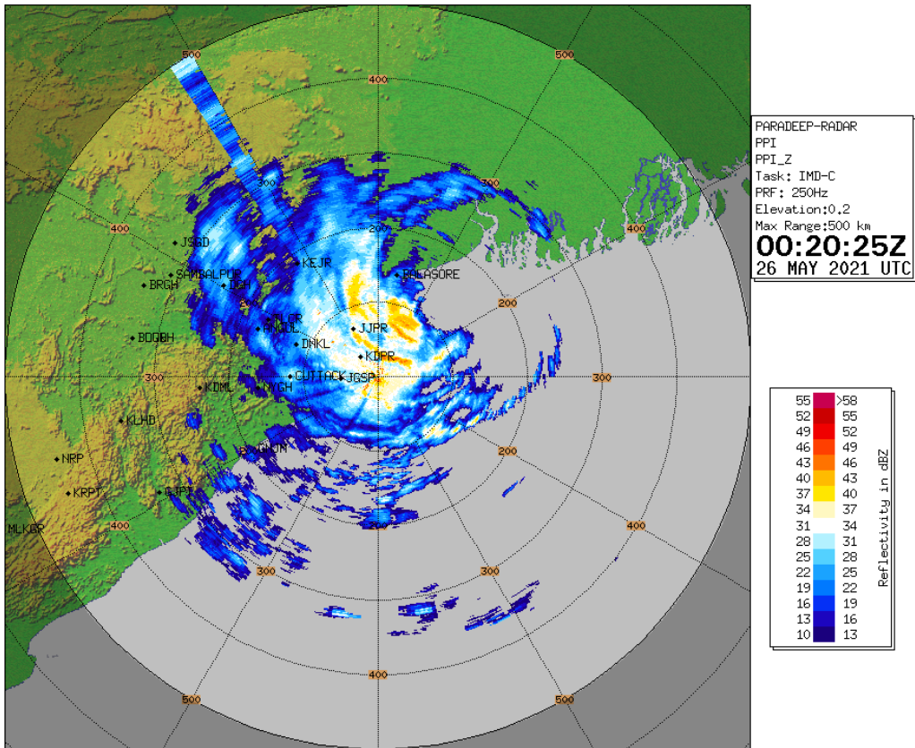
Latest imagery from Doppler Weather RADAR Paradip
